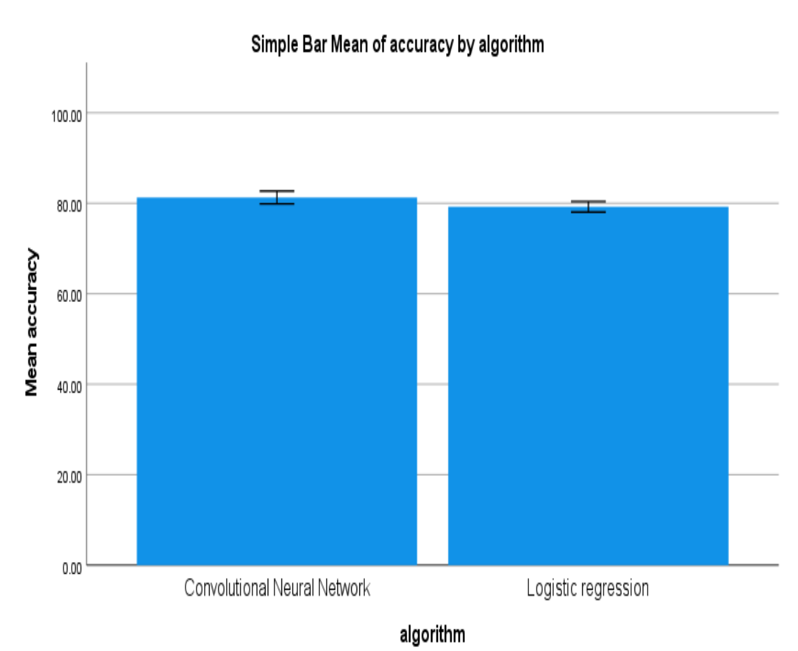
CNN vs Logistic Regression
